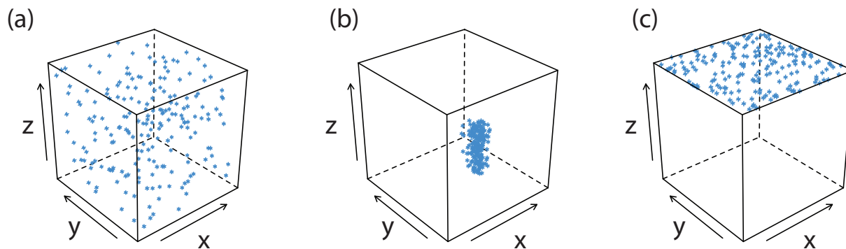
Figure 8.4 Three examples of impurities that may form during precipitation. The cubic frame represents the precipitate and the blue marks are impurities present as (a) inclusions, (b) oclusions, and (c) surface adsorbates. Inclusions are randomly distributed throughout the precipitate. Oclusions are localized within the interior of the precipitate and surface adsorbates are localized on the precipitate's exterior. For ease of viewing, in (c) adsorption is shown on only one surface.
